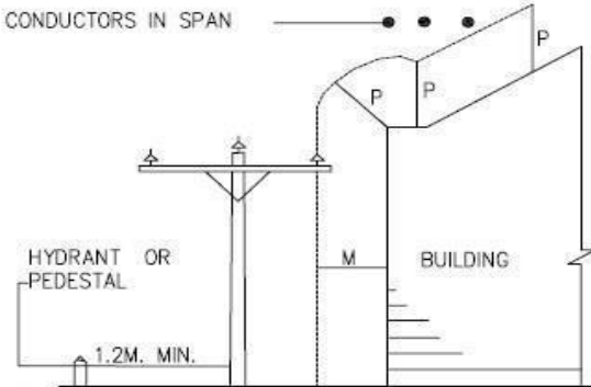
MINIMUM CLEARANCE FROM BUILDINGS
