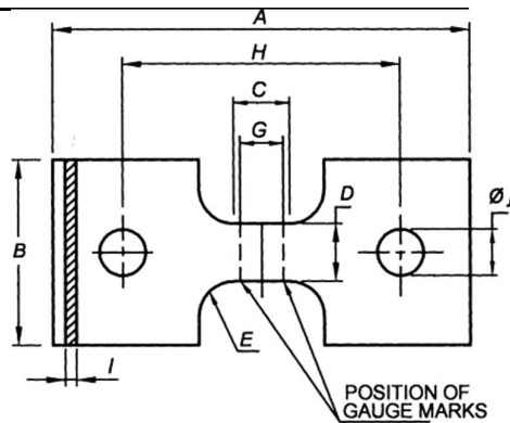
FIG. 6 TYPE 3 TEST PIECE
