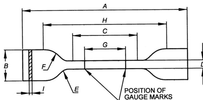
FIG. 5 TYPE 2 TEST PIECE
