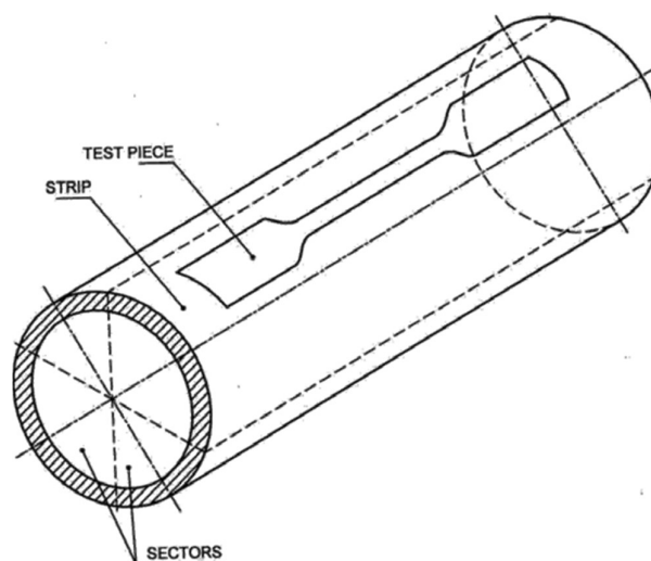
FIG. 7 PREPARATION OF TEST PIECES
