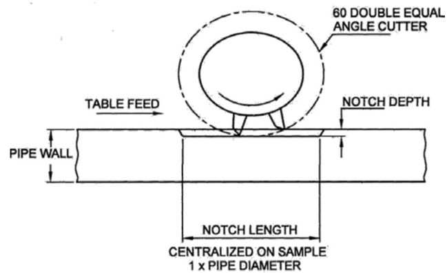
FIG. 8 NOTCH METHOD
