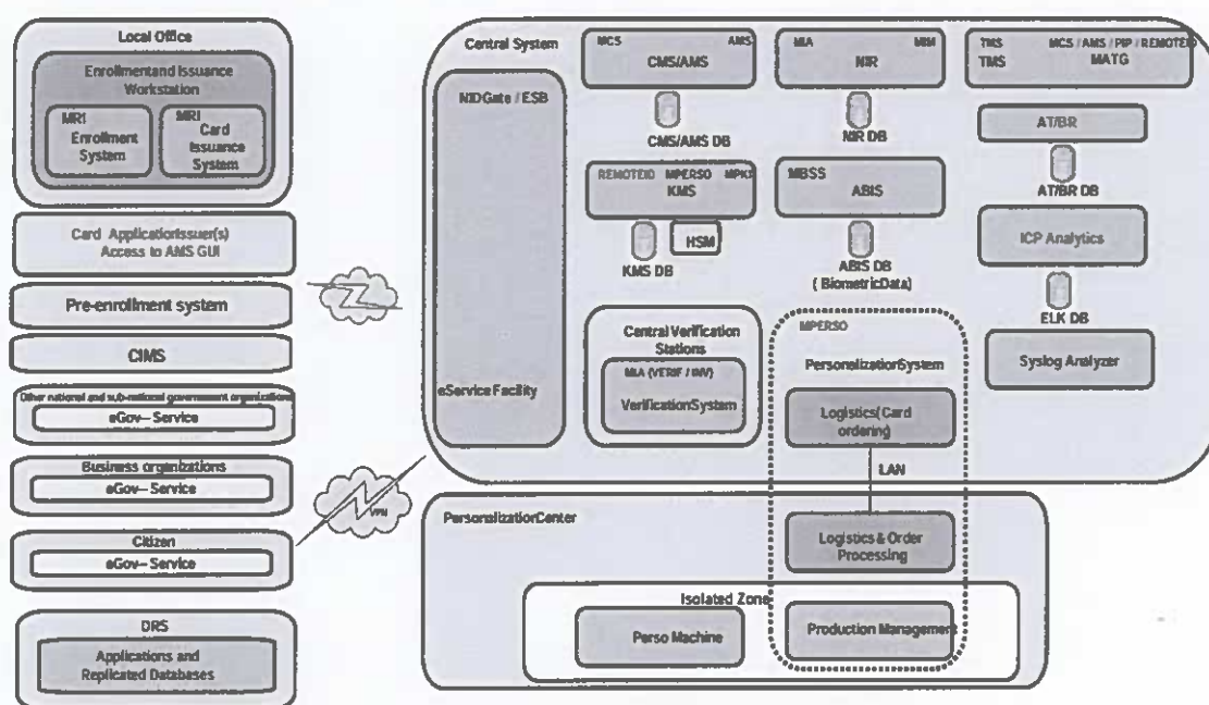
Logical view of NIDMIS System
