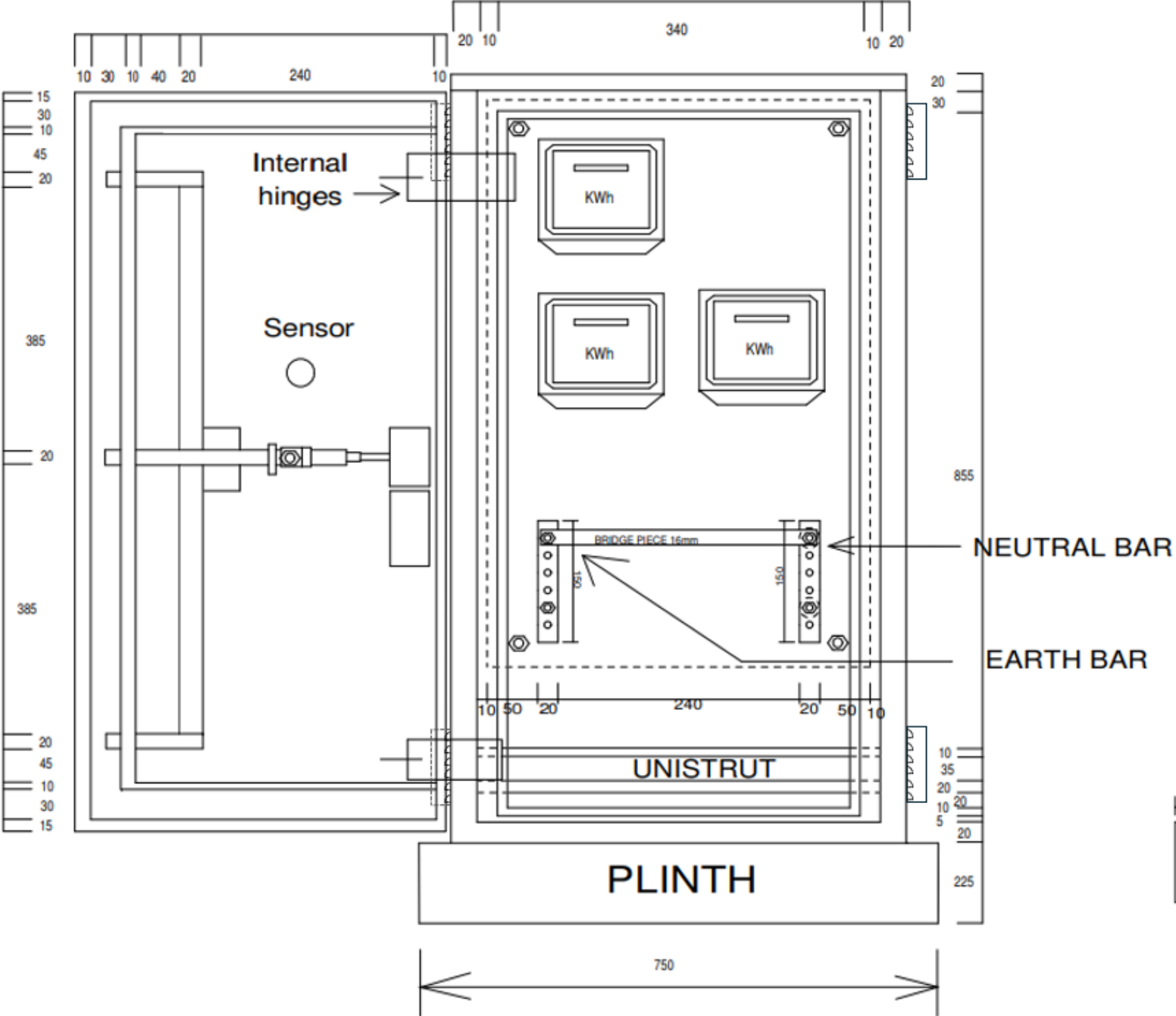
FRONT VIEW WITHOUT DOOR
