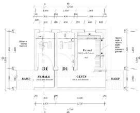
GROUND FLOOR PLAN LAYOUT
