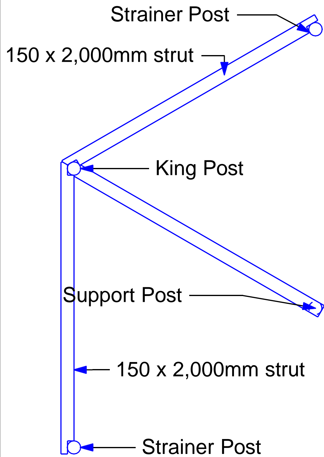
CORNER STRAINER ASSEMBLY PLAN
