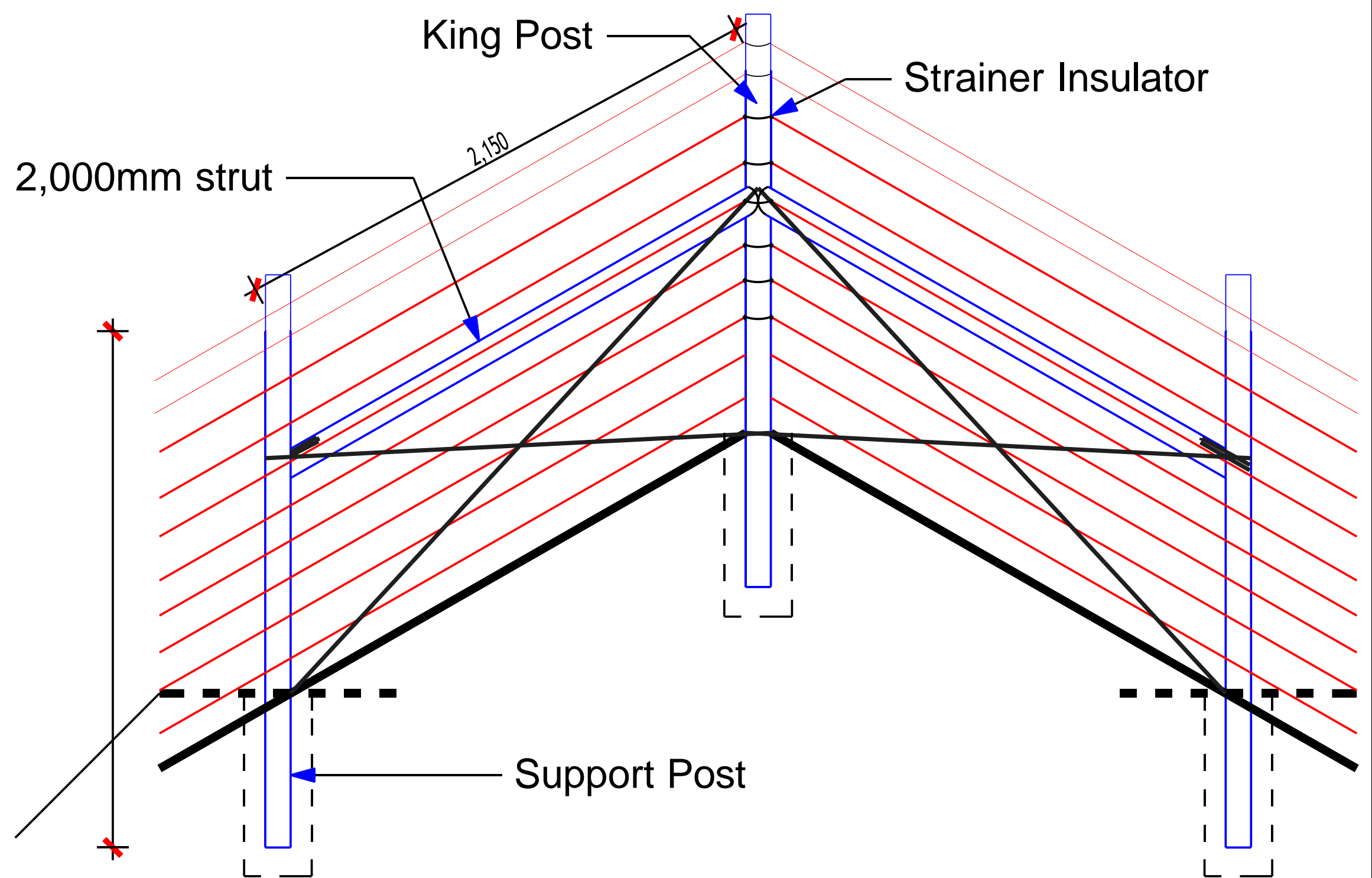
CORNER STRAINER ASSEMBLY
